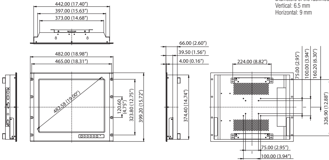
Panel Cut-out Dimensions: 444 x 376.4 mm (17.48\"/>
