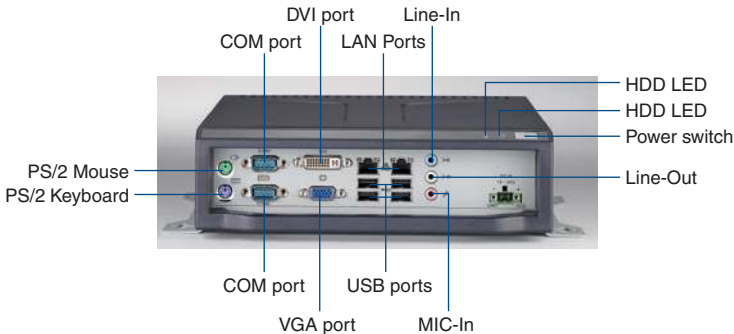
ARK-6310-6M01E Front IO view
